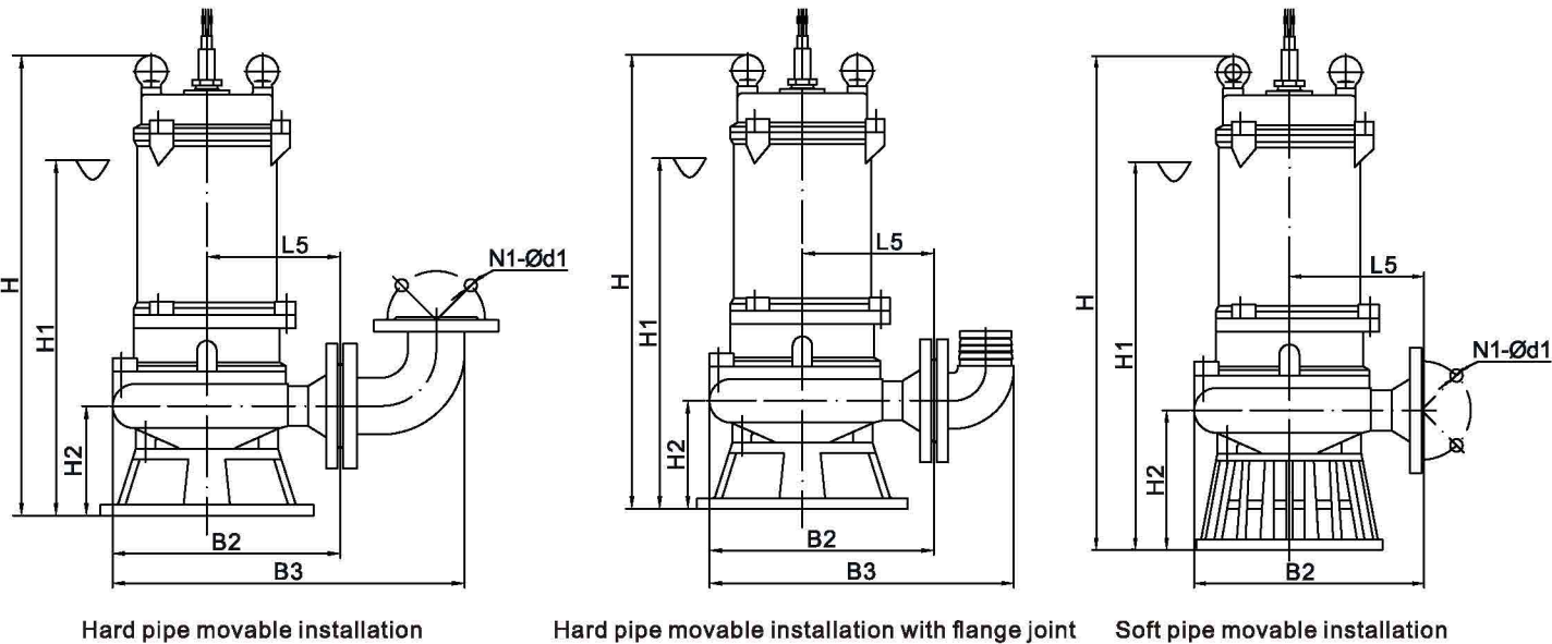
Movable installation
