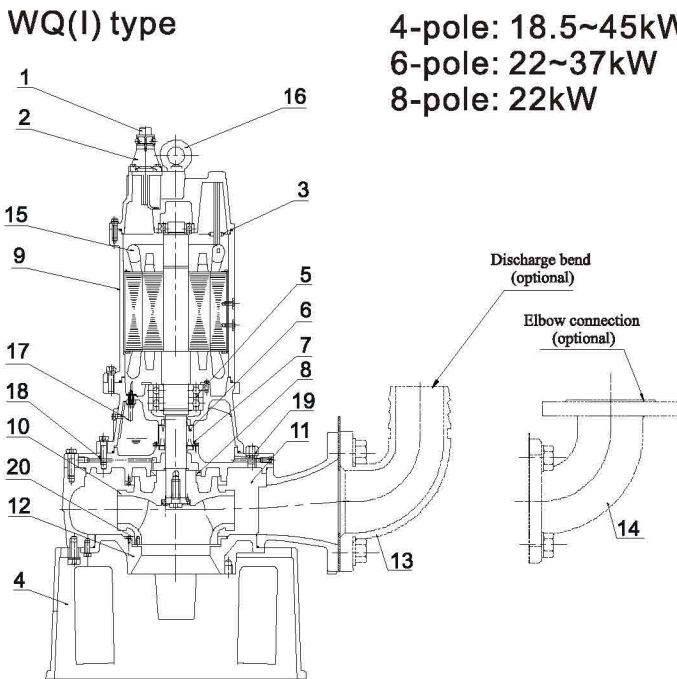
Sectional drawing of sewage pump with 4,6,8 pole motor
