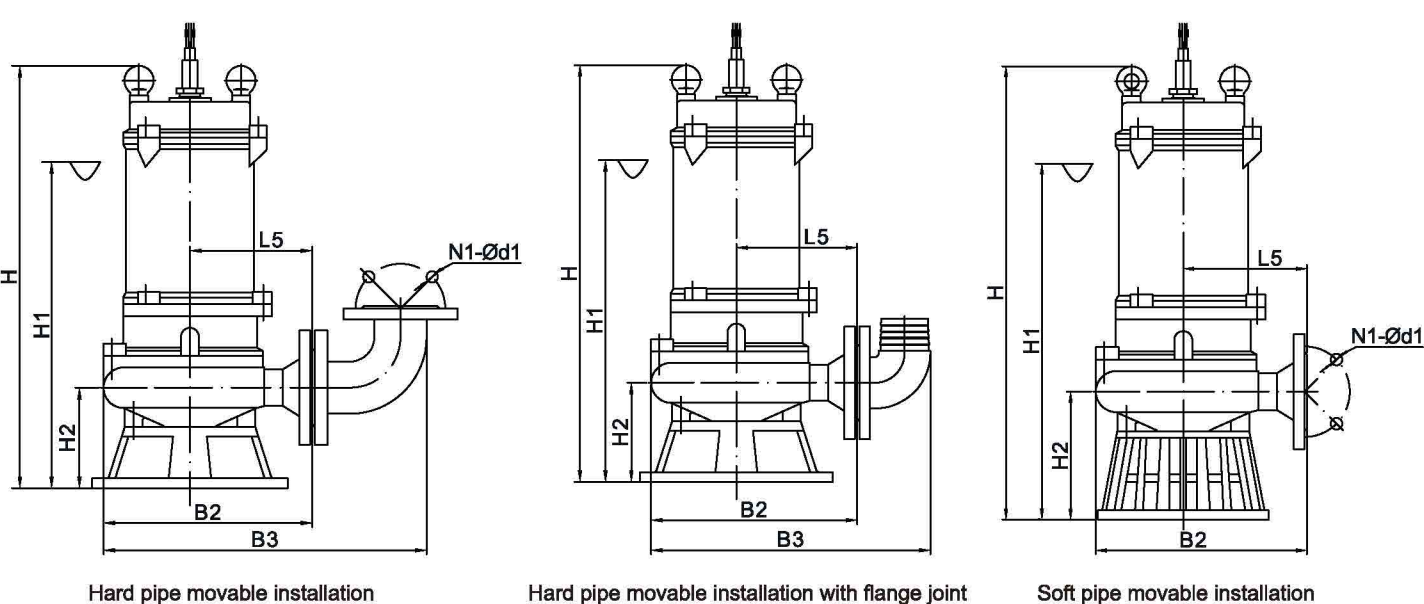
Movable installation
